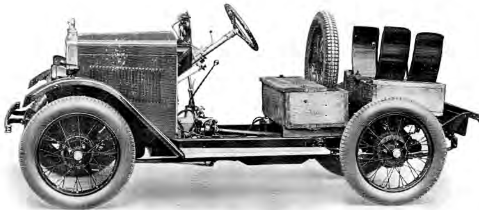
The MORRIS MINOR CHASSIS Price £100 Ex Works
