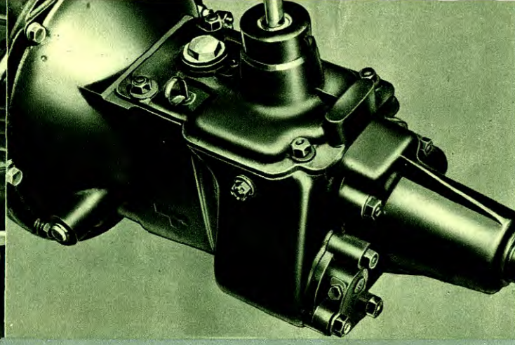
The new four-speed gearbox has silent helical gears and synchromesh engagement on second, third and top gears. In addition the driven shaft is supported on three bearings.
