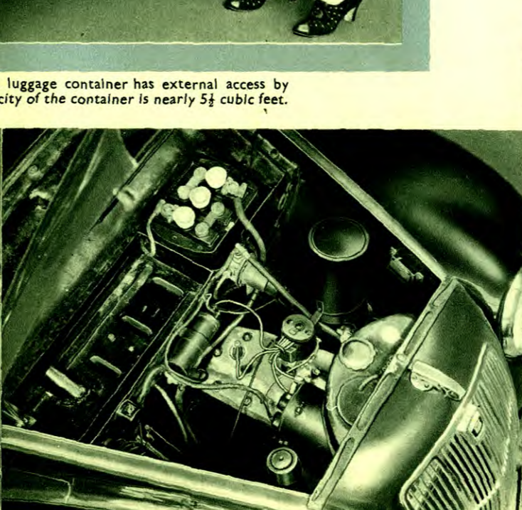
The power unit has been considerably improved by the provision of a balanced crankshaft, tin-coated aluminium pistons, improved manifolding and improved lubrication. All maintenance adjustments are easily accessible.
