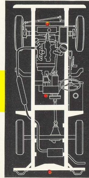
Rear power take-off drive section for operating, through a splined shaft, machinery towed by the vehicle.
