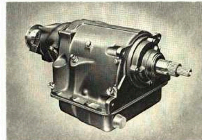
AUTOMATIC TRANSMISSION. Borg Warner Model 8—extensively tested and proven—to match the high torque of the Jaguar 4.2 litre engine. D1/D2 dual drive range gives smooth shifts and option of first or second gear starts as well as full engine braking.
